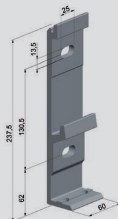
Plaque murale auxiliaire
