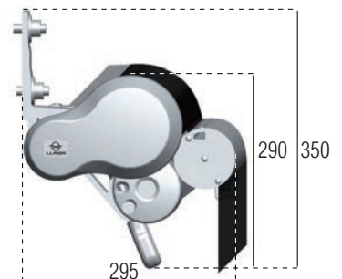
Installation SCDV
